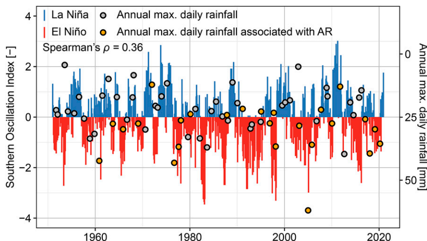
FIG. 6. The SOI and annual maximum daily rainfall teleconnection for the LVW watershed. Events associated with atmospheric rivers (ARs) are highlighted in orange.
