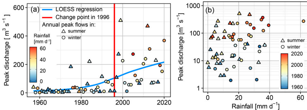
FIG. 2. (a) Annual peak flows for the LVW watershed over the 1957–2020 period and (b) their corresponding daily rainfall totals. Blue and red lines in (a) represent the locally weighted polynomial regression (LOESS; Cleveland 1979) and Pettitt test changepoint fitted to all annual peak flows, respectively. Peak flows in both subplots are distinguished by their season.
